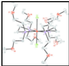
Fig. 1. The structure of the title compound with 50% probability displacement ellipsoids and the atom-numbering scheme. The H atoms are omitted for clarity.
